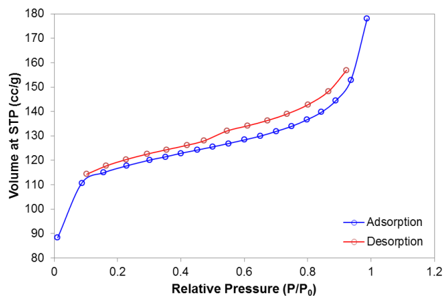
Figure S3. Nitrogen sorption isotherms performed on 1 at 77 K reveal a Brunauer-Emmett-Teller surface area of 370(5) \text{ m}^2 \text{ g}^{-1} .
