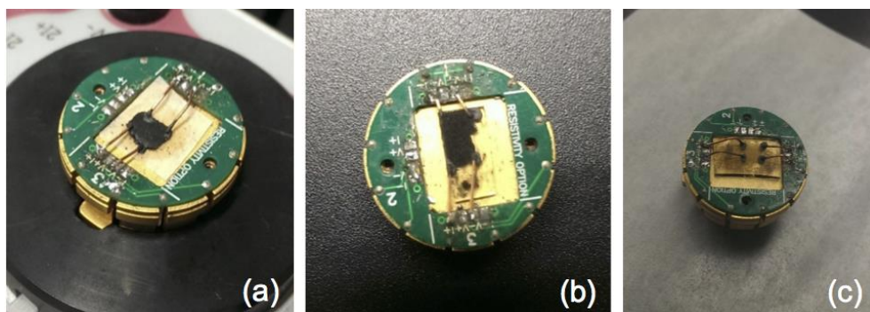
Figure S14. Images of the samples – pellet (a) or films of 1 (b) and (c) – and their puck assemblies for conductivity measurements. Graphitic carbon paint was used to create Ohmic contacts.
