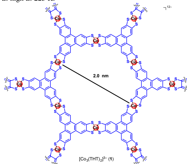
Figure 1. Framework of the 2D cobalt dithiolene framework [\text{Co}_3(\text{THT})_2]^{3-} , 1 , studied here.
