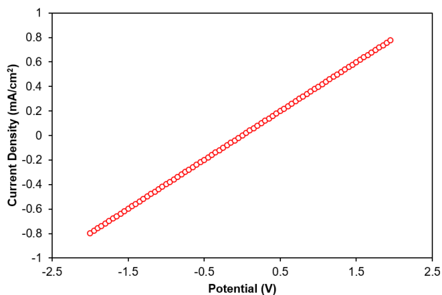
Figure S5. Room temperature I-V trace of solid 1 pressed in a pellet of 0.24(2) \text{ mm} thickness, which displays Ohmic response between -2.0 and +2.0 \text{ V} .
