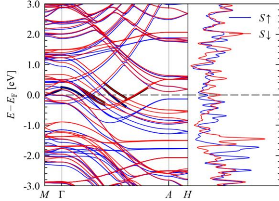
Figure S26. Calculated electronic dispersion and density-of-states curve for Framework 1 with a charge of -3 e per unit cell. As in Figure S24, the blue and red lines show the spin-up and spin-down components of the electronic structure, respectively, and the overlaid black lines illustrate the fitting to estimate the carrier effective masses.
