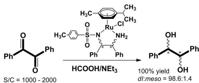
Figure 7. Noyori asymmetric hydrogenation of benzil with ruthenium catalyst yields hydrobenzoin in a high diastereomeric and enantiomeric purity.
