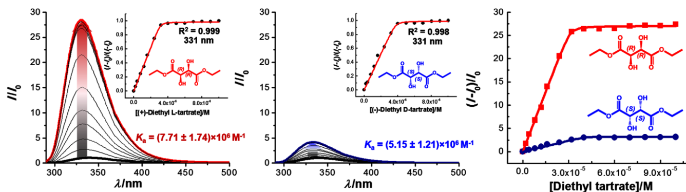
Figure 3. Fluorescence titrations of L-tryptophan - FPBA (1:1, 40 \mu\text{M} ) with diethyl-tartrate enantiomers (0-100 \mu\text{M} ) in MeCN. \lambda_{ex} = 280 \text{ nm} . Left: (+)-diethyl-L-tartrate; Center: (-)-diethyl-D-tartrate; Right: Isotherms show the difference in signal amplification for the two diethyl tartrate esters ( \lambda_{em} = 330 \text{ nm} )
