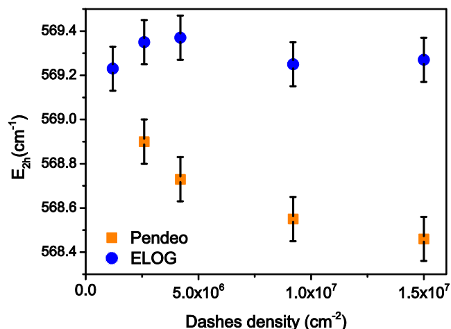
Fig. 9. E_2^H phonon mode peak position measured by Raman spectroscopy on ELOG and pendeo samples as a function of dash density.
