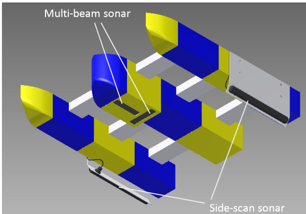
Fig. 1. Rendering of a trimaran hull structure with locations of the side-scan and multi-beam echo-sounder labelled. All structural components are either 3D printed or laser cut.
