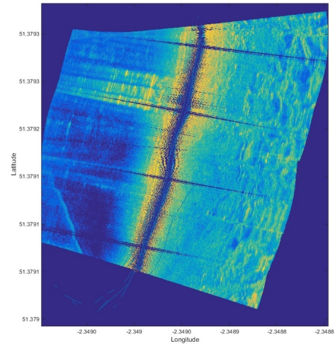
Fig. 3. Co-registered GPS and side-scan sonar data, collected by the catamaran vessel of Figure 2 in the Kennet and Avon Canal in Bath, UK
