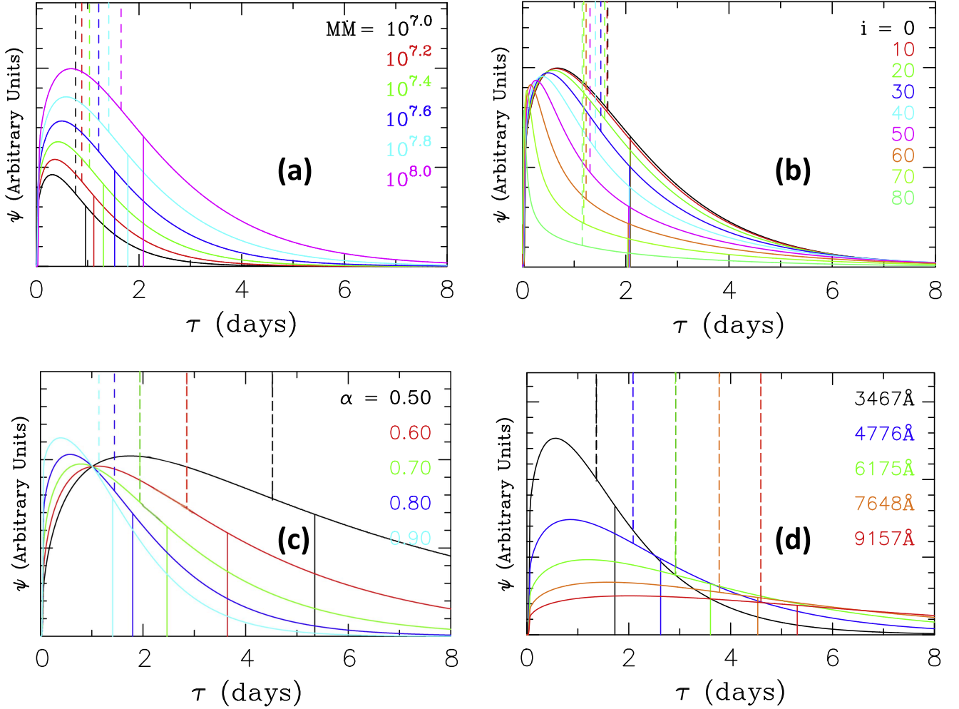
Figure 1. Accretion-disk response functions for varying M\dot{M} (a), inclination (b), temperature profile slope (c), and wavelength \lambda (d). When not varied, the values are set to \lambda = 4000 \text{ \AA} , i = 0 , \alpha = 0.75 , and M\dot{M} = 10^8 M_{\odot}^2 \text{ yr}^{-1} . Solid and dashed lines indicate the mean and median response function delays, respectively. Panel (b) shows that the mean delay \langle \tau \rangle is inclination independent.
