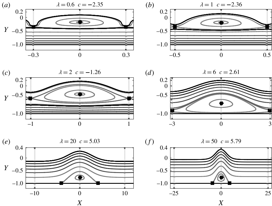
FIGURE 6. Phase portraits with H=0.4 , \gamma=10 and varying the wavelength with \lambda=0.6 , 1, 2, 6, 20, 50. The black markers depict the stagnation points as before. The thick black curve is at \psi(X, Y)=0 . It should be noted that these solutions have different wavelengths from those in figure 5 and therefore correspond to different wavelength regimes: from short waves to long waves, from (a–f).
