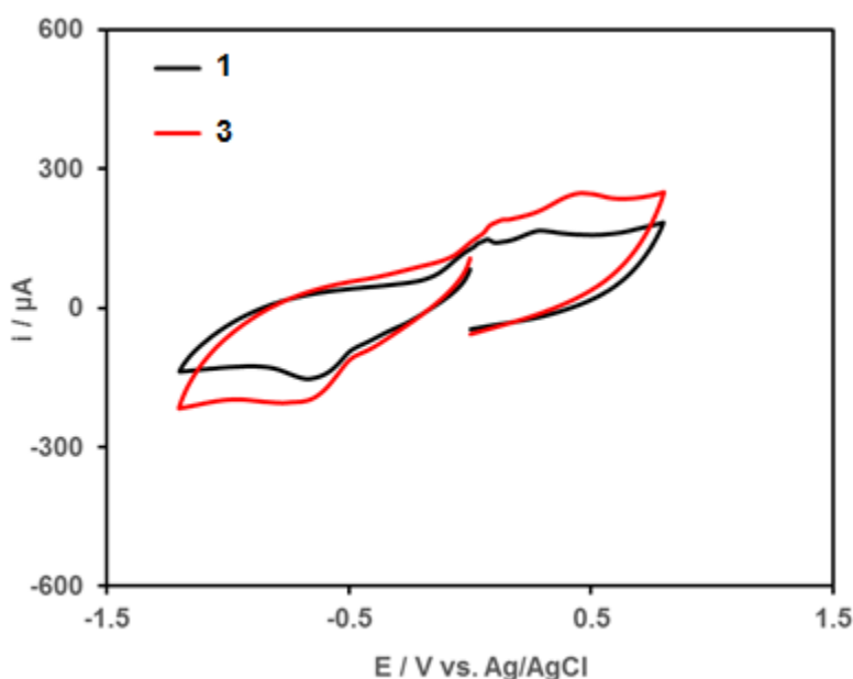
Figure 6. The cyclic voltammograms of complexes 1 and 3 in 0.05 M LiClO 4 -Acetonitrile at a scan rate of 5 mV s -1 .
