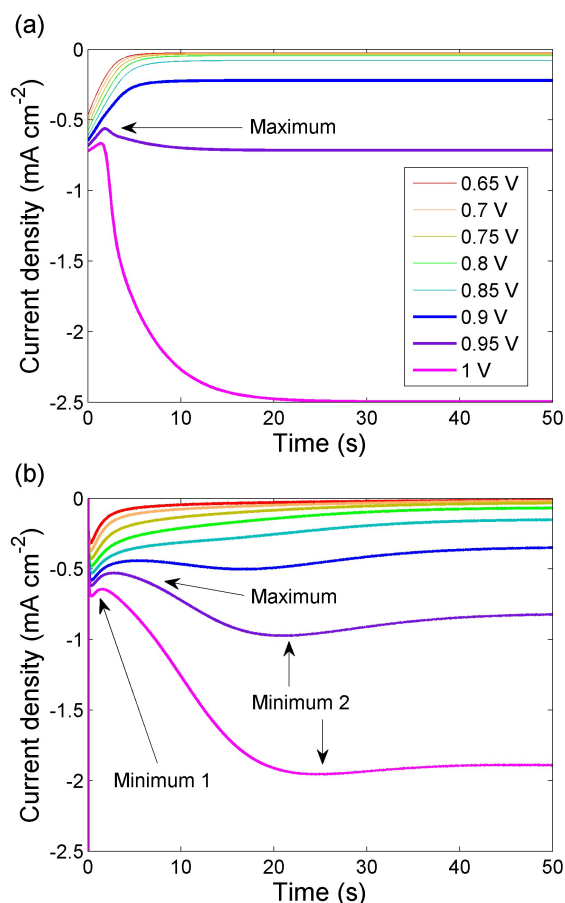
Fig. 5 (a) Simulated and (b) measured evolution of current density over 50 s following a jump from 0 V to V_{jump} in the dark, for varying different values of V_{jump} at room temperature (298 K). This gives good qualitative agreement between theory and experiment.
