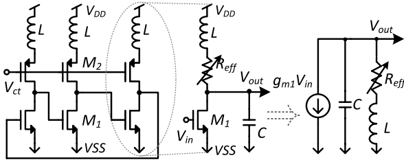
Fig. 2. Addition of peaking-inductor with RO-VCO.
