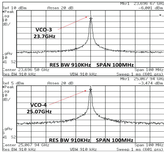
Fig. 6. The spectrum of highest oscillation frequency of VCO-3/4.
