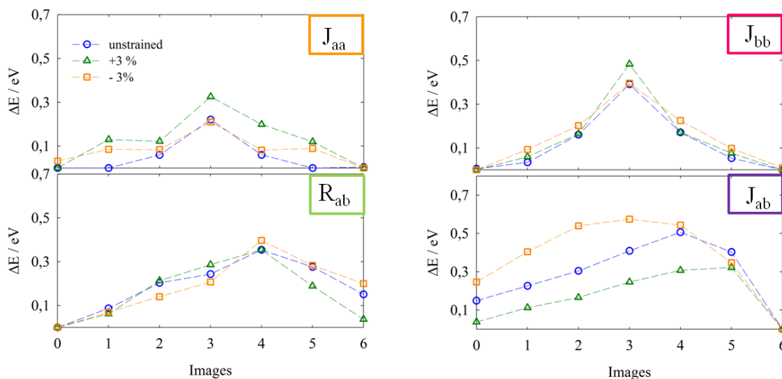
Figure S5 – Energy barriers profile obtained from NEB calculations for the compressive (orange squares), zero (blue circles) and tensile (green triangles) strain for the different jumps and rotations described in Figure 5 of the main text.
