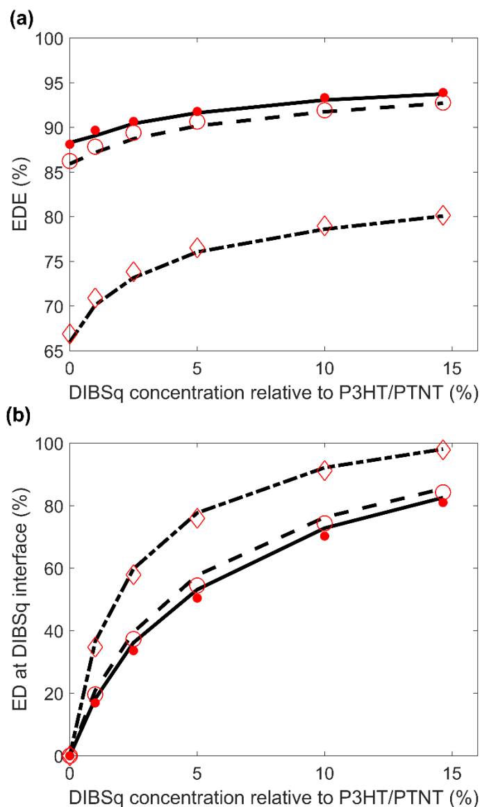
Figure 7. (a) EDE as function of DIBSq content for a P3HT:PCBM:DIBSq (black) and PTNT:PCBM:DIBSq (red) BHJ with a feature size of 14 nm (solid line/dots), 15 nm (dashed line/open circles) and 31 nm (dash-dot line/diamonds). The number of excitons that dissociated at the DIBSq interface is also shown as a function of DIBSq content in (b).
