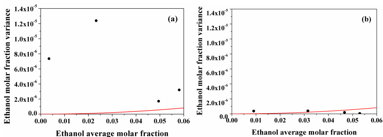
Figure 3 – Variances of ethanol molar fractions for catalytic reactions (●) and chromatographic measurement fluctuation model (-) as functions of ethanol average molar fractions for catalysts MgO-SiO 2 -(50:50) (a) and MgO-SiO 2 -(95:5) (b).
