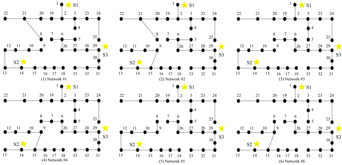
Fig. 9 Possible network topology caused by different tie line allocation
