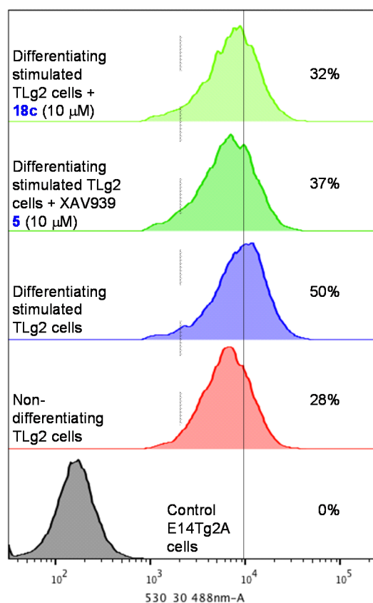
Figure 4. Flow-cytometric analysis of TLg2 cells (and E14Tg2A control cells) grown under the indicated culture conditions. The black line indicates the median GFP fluorescence intensity of TLg2 cells cultured for 3 d in the presence of N2B27 medium and % is the percentage of cells found with fluorescence above that level under the various conditions.
