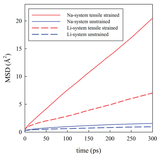
Fig. 6 Mean square displacement (MSD) vs. time for \text{Li}_{0.9}\text{FePO}_4 (dashed lines) and \text{Na}_{0.9}\text{FePO}_4 (solid lines).
