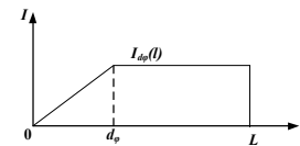
Fig. 6 Triangular-rectangular distribution of demand currents on phase \phi
