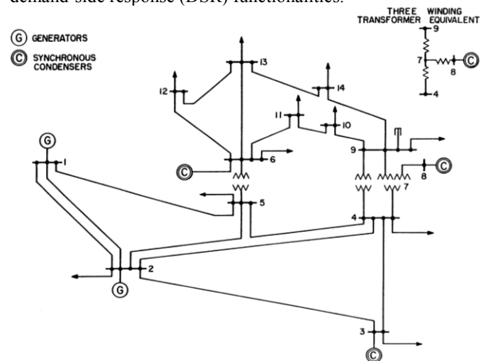
Fig. 1. Original IEEE 14-bus test system [1, 2].
