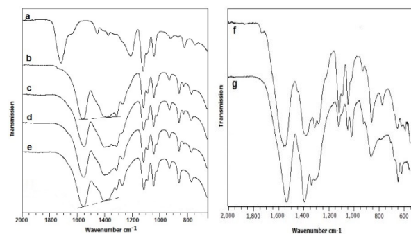
Fig. 1. FT-IR of (a) lactic acid ; (b) \text{CaMn}_2\text{Ox-lactate} ; (c) \text{CaMn}_3\text{Ox-lactate} ; (d) \text{CaMn}_4\text{Ox-lactate} ; (e) \text{Mn}_3\text{O}_4\text{-lactate} ; (f) Co:lactate 1:2; (g) Co-lactate 1:1. Dotted lines show increase in relative intensity of \nu_{\text{s}} ( \text{CO}_2^- ) absorbance band at \sim 1400\text{ cm}^{-1} with \text{Ca}^{2+} content.
