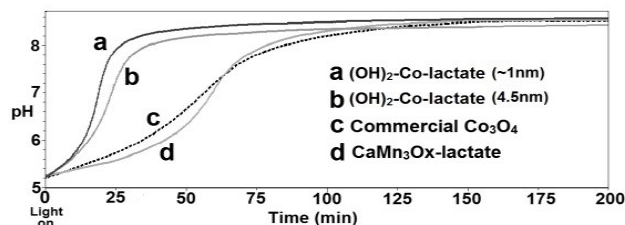
Fig. 5. Change in pH for a photocatalytic water oxidation utilizing [Ru(bipy) 3 ]Cl 2 2+ , [Co(NH 3 ) 5 ]Cl 2 2+ (electron acceptor) and catalyst suspended in N 2 degassed aqueous acetate buffer solution at pH 5.2. Time course using Co-lactates, CaMn 3 Ox-lactate, and commercial Co 3 O 4 (with 10mg metal oxide present in all cases).
