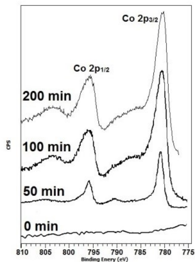
Figure 9. High resolution XPS analysis of CaMn 3 Ox-lactate catalysed photocatalytic reaction with washed samples recovered at intervals showing accumulation of Co from decomposed electron acceptor. The Co2p region has band position and shape consistent with cobalt oxide as Co 3 O 4 together with broader bands of increasing intensity indicating increasing hydroxide presence.
