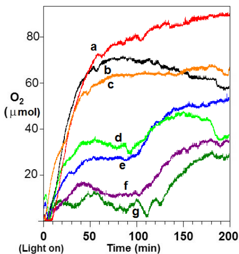
Fig. 4. Graph of O_2 release with time for water oxidation reactions using a commercial Co_3O_4 nanopowder and a range of chelated metal oxide catalysts. (a) Co:lactate 1:1; (b) commercial Co_3O_4 ; (c) Co:lac 1:2; (d) CaMn_3O_x -lactate; (e) Mn_3O_4 -lactate; (f) CaMn_4O_x -lactate; (g) CaMn_2O_x -lactate.
