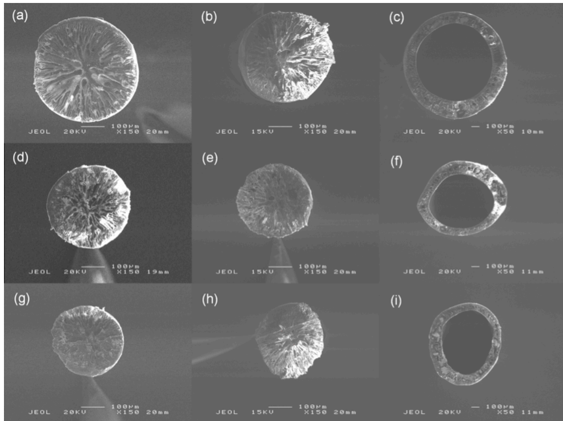
Figure 2. SEM images of PLGA 65:35 fibres and effect of drug release in distilled water.
