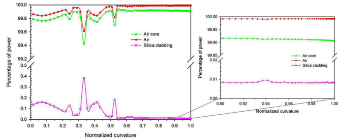
Fig. 6. Percentage of optical power in the air core (green line with “x”), in all the air holes of the fiber (red line with filled dots) and in the silica struts of the cladding (purple line with empty dots). On the right hand side is a magnification of the plot for curvature values between 0.9 and 1 [45].
