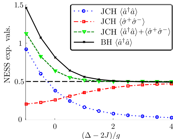
Figure 4. NESS particle numbers per resonator for sixteen-site Bose-Hubbard and Jaynes-Cummings CRAs driven at their single particle resonances. Parameters: photonic driving \Omega/\gamma_p = 2 , atom-resonator coupling strength g/\gamma_p = 20 , photon hopping rate J/\gamma_p = 1 . Trajectory calculations retain p = 6 photons per resonator for the BH simulation, and p = 5 for the JCH. Each Jaynes-Cummings detuning \Delta/g is mapped to an effective Kerr nonlinearity via Eq. (6) to enable a comparison.
