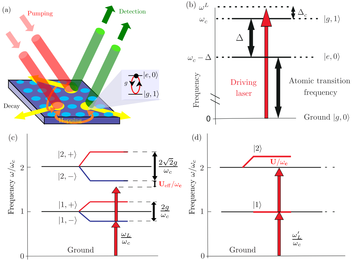
Figure 1. (a) A schematic of a three site set up. Here two-level systems are embedded in cavities in a 2D photonic crystal but alternative implementations involving Circuit QED architectures could be also envisaged [18]. Coherent photon hopping between cavities results from modal overlap between neighboring cavities and photons can be lost due to decay mechanisms. (b) The relevant frequency scales and detunings used to describe a driven Jaynes-Cummings resonator. (c) The low-lying eigen-levels for the Jaynes-Cummings interaction, showing the definition of the effective Kerr nonlinearity U_{\text{eff}} . (d) The low-lying excitations of a Kerr-nonlinear resonator. Arrows schematically show that a driving laser resonantly exciting a single-particle mode from the ground state is detuned from higher modes. Solid horizontal lines represent multiples of the cavity frequency. Dotted horizontal lines are a guide to the eye.
