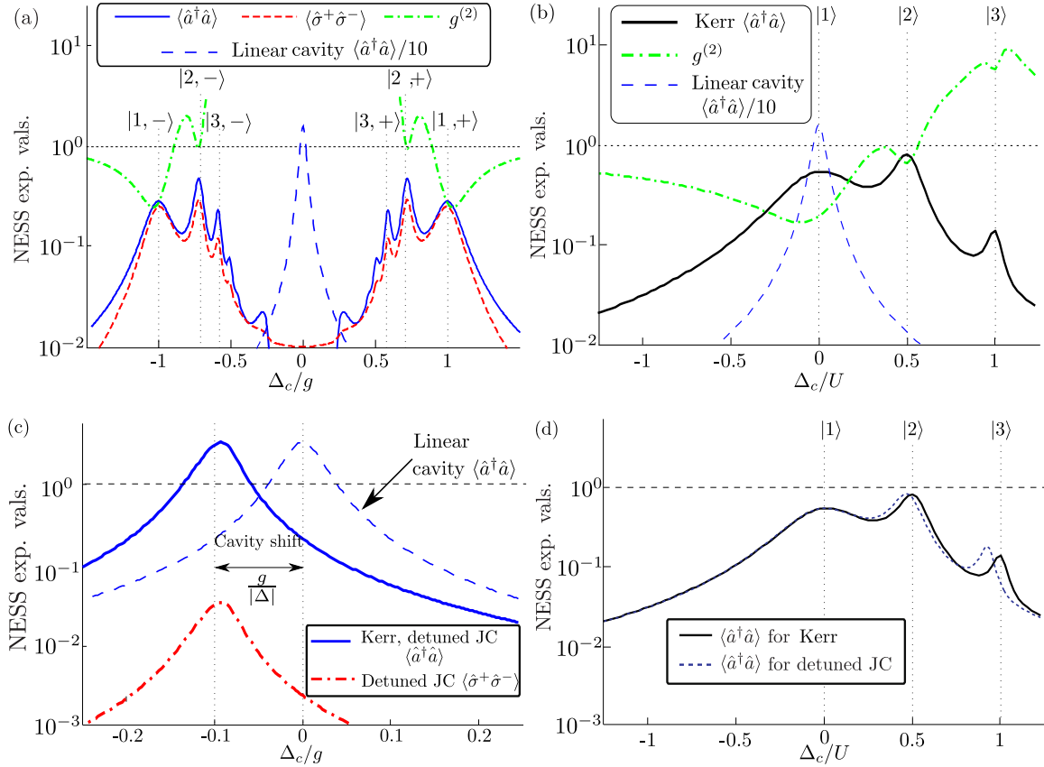
Figure 2. Steady state values of photonic/atomic population (solid/dashed line) and the second order photon correlation function ( g^{(2)} , dot-dashed line) as a function of the driving laser-cavity detuning for a single driven dissipative resonator. (a) Jaynes-Cummings resonator (atom resonant with the cavity mode \Delta/g = 0 ). The central Lorentzian (dashed curve) is the response of an empty (linear) driven-dissipative resonator \langle \hat{a}^\dagger \hat{a} \rangle / 10 . (b) Kerr-nonlinear resonator. Vertical dashed lines and labels in both plots indicate resonator resonances according to Eqns. (3) and (4), respectively. Parameters: Both systems share \Omega/\gamma_p = 2 . Jaynes-Cummings coupling g/\gamma_p = 20 . For the Kerr resonator: U/\gamma_p \approx 11.7 , set using Eq. (6). (c) The response of a far-detuned ( \Delta/g = -10 ) Jaynes-Cummings resonator for identical atom-resonator coupling, driving and loss as above (d) Comparison of the Kerr response in (b) and that of a detuned Jaynes-Cummings resonator ( \Delta/g = -10 ) with an ultra-strong nonlinearity g'/\gamma_p \approx 1.6 \times 10^4 .
