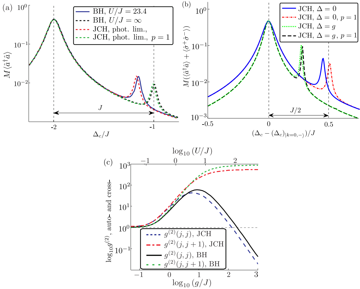
Figure 5. (a) The one and two particle peaks (right and left features, respectively) for a homogeneously driven three-resonator BH model in the strongly nonlinear regime (solid blue, U/J = 23.4 ), and the hard core limit ( p = 1 , dotted black). Spectra for larger U approach the hard core limit asymptotically. Parameters: photon hopping rate J/\gamma_p = 20 , driving \Omega/\gamma = 0.5 . Also shown are results for a strongly detuned JCH system operating in the photonic limit with \Delta/g = -10 , and an unrealistically large atom-resonator coupling g/\gamma_p \approx 2 \times 10^5 . (b) Analogous photon number spectra for the JCH model with g/\gamma_p \approx 800 (chosen according to Eq. 6), and the photon driving and tunneling rates as in (a), for two different atom-resonator detunings \Delta/g (dashed and dash-dotted). Again, the hard-core spectra are recovered in the limit g \rightarrow \infty . The horizontal axis is taken relative to the single particle spectral position (\Delta_c)_{|k=0,-} , different for each \Delta . (c) The auto- and cross-photon correlation functions measured at the two particle peak as a function of the nonlinearity in both the BH and JCH ( \Delta = 2J ) Hamiltonians. JCH systems with different couplings g are compared with Bose-Hubbard systems whose strength U = U(g) (see upper horizontal axis) is obtained from Eq. 6. Note these calculations are performed at the lower driving \Omega/\gamma_p = 0.25 , to avoid truncation errors at low nonlinearity.
