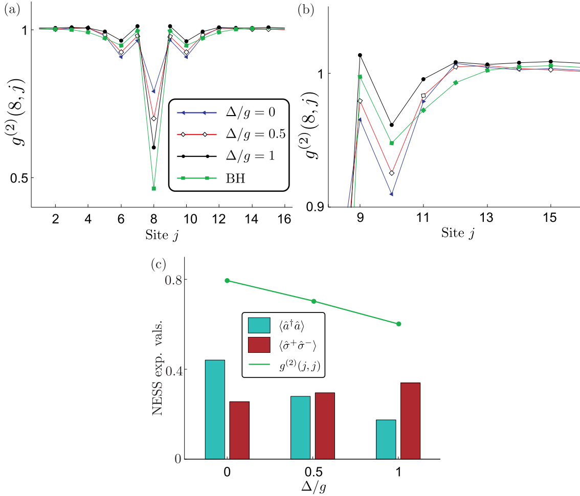
Figure 6. (a) Steady state photon density-density correlations for a cyclic 16 site JCH system, driven by lasers exciting the \pi/2 momentum mode of the system. Thin lines between markers are drawn to guide the eye. Parameters: hopping J/\gamma_p = 2 , atom-resonator coupling g/\gamma_p = 10 , driving strength |\Omega_k|/\gamma_p = 2 . Also shown (solid green) are density-density correlations for a M = 16 site system with ‘matched’ Kerr nonlinearity U/\gamma_p \approx 6 in each resonator, and otherwise identical parameters. (b) Closer view of the correlation functions. (c) The relative atomic and photonic population in each resonator in the steady state for the three different values of atom-resonator detuning chosen, as well as the on-site photon correlation function.
