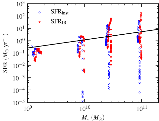
Figure 4. SFR versus M_* for the major merger simulations. The blue circles indicate that the true instantaneous SFR is used, whereas the red triangles indicate that the SFR value is inferred from L_{\text{IR}} . In both cases, the true M_* is used (but for clarity, the M_* values for the red triangles have been increased by 0.03 dex). The solid black line is the best fit to the z \sim 0.2\text{--}0.4 star-forming galaxies of Karim et al. (2011). For the recently quenched galaxies, the inferred and actual locations in the SFR– M_* plane differ significantly (i.e. there are many blue circles that lie significantly below all of the red triangles).
