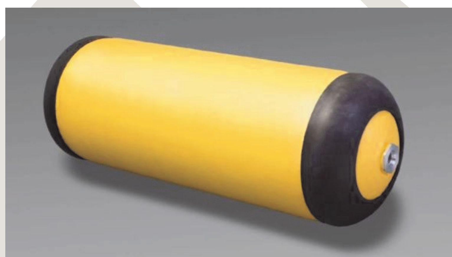
Figure 1: 70 MPa hydrogen tank used in the Toyota Mirai fuel cell vehicle [3]
