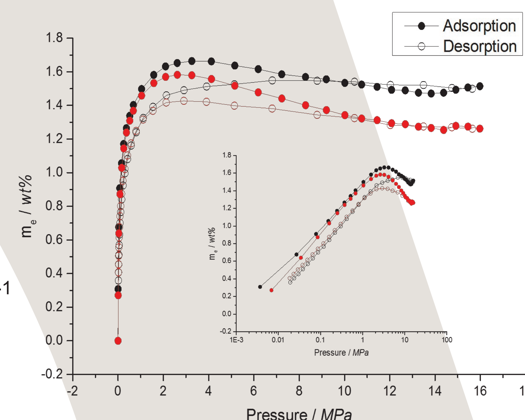
Figure 5: High Pressure (160 bar) Hydrogen adsorption isotherms at 77 K for PIM-1 powder (black) and PIM-1 film (red)
