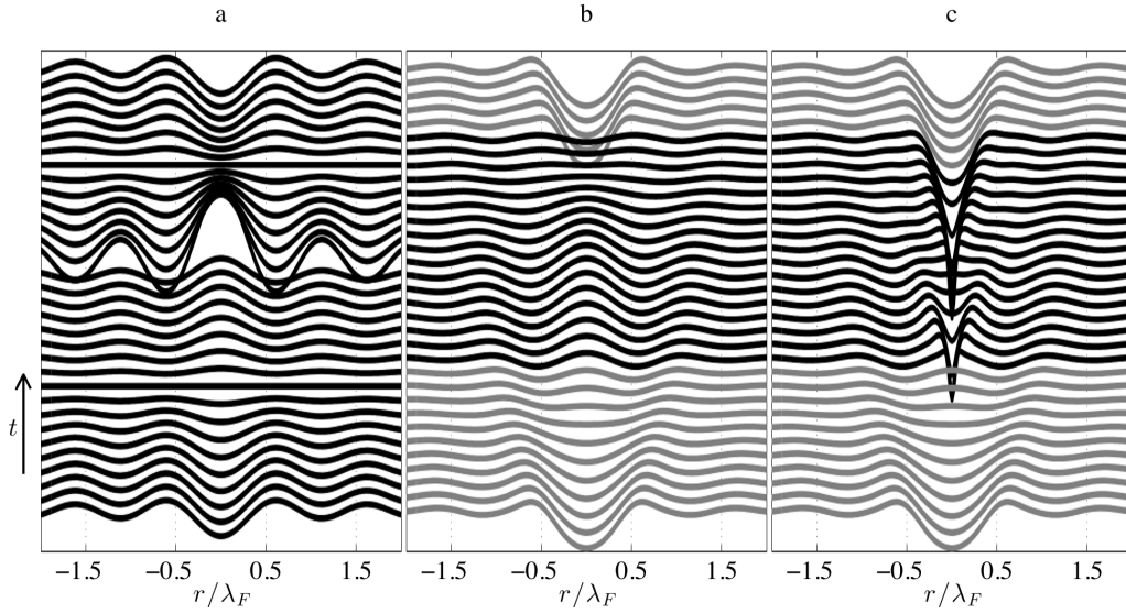
FIGURE 11. The time evolution of the free surface through the course of a Faraday period for the same bouncer as in figure 8. (a) The model of Moláček & Bush (2013b), as described by equation (3.10). The discontinuity arises when the surface is updated by the addition of a new Bessel function. (b) Our model's prediction, \bar{\eta} , for the free surface in the absence of the current impact. The dark curves correspond to wave forms arising when the drop is in contact with the bath, the lighter curves to times when the drop is in flight. (c) Our model prediction for the free surface when the current droplet impact is included.
