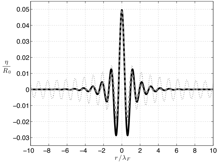
FIGURE 9. Comparison between the wave-field predictions of the present model (black curve) with those of Moláček & Bush (2013b) without (dotted curve) and with (grey dashed curve) the higher order spatial damping correction suggested by Moláček & Bush (2013b) to the Bessel model (3.10).
