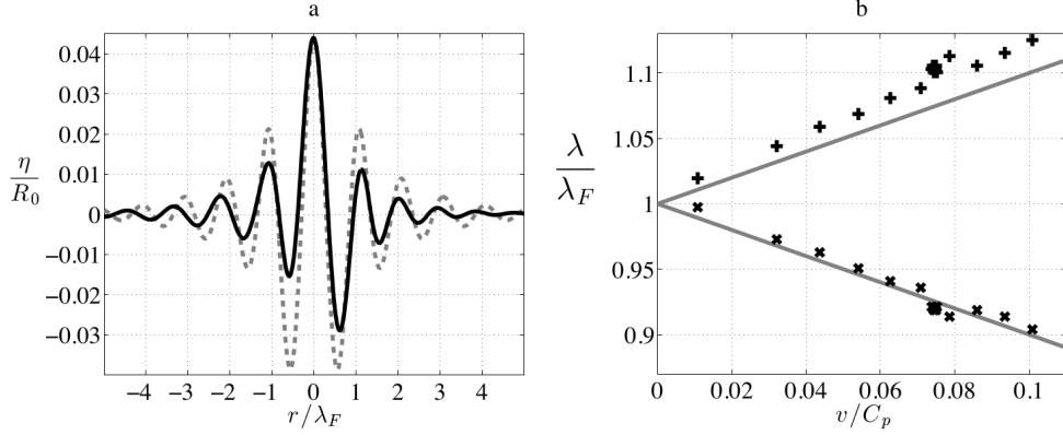
FIGURE 12. (a) The Doppler effect arising at \Omega = 0.8, \Gamma = 3.6 . The solid line shows the surface along the direction of motion, the dashed line that in the transverse direction. The horizontal axis is in units of Faraday wavelengths, and the vertical axis in units of drop radii. (b) The Doppler effect displayed ahead and behind the walker, with \lambda/\lambda_F (vertical axis) in terms of V/C_p . The \times markers depict the wavelength ahead of the walker, the + markers the wavelength behind it. The lines indicate the magnitude of the Doppler effect reported by Eddi et al. (2011). V is the mean walker speed and C_p the phase speed.
