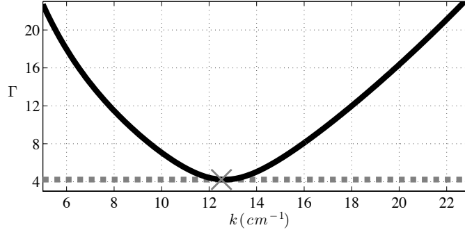
FIGURE 1. Approximate Faraday subharmonic stability curve (black) as predicted by (2.35) for the experimental parameters in Appendix B. The viscosity of the fluid \nu was adjusted to \nu^* = 0.8025\nu so that the minimum of \Gamma(k) , as predicted by (2.35), matches the experimental value \Gamma = 4.22 reported in Wind-Willassen et al. (2013) and shown by the horizontal line. The minimum is achieved at k_F = 12.64\text{cm}^{-1} . The \times indicates the numerically observed critical value for instability of (2.33), specifically k_* = 12.52\text{cm}^{-1} at \Gamma = 4.22 . The inverse Reynolds number for this case, based on \nu^* , the Faraday frequency of \omega_0/2 and the associated Faraday wavelength \lambda^* , is \epsilon \approx 0.016 .
