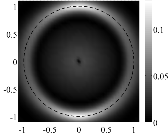
FIGURE 13. Amplitude of the Fourier spectrum of the computed wave field for a walker immediately before the drop impacts the surface. A superposition of Bessel functions J_0(k_F r) would have a spectrum only on the dashed circle of radius k_F . It is the frequency spread of the spectrum about this circle that allows for a Doppler shift in the wavefield. Axes are in units of inverse Faraday wavelengths.
