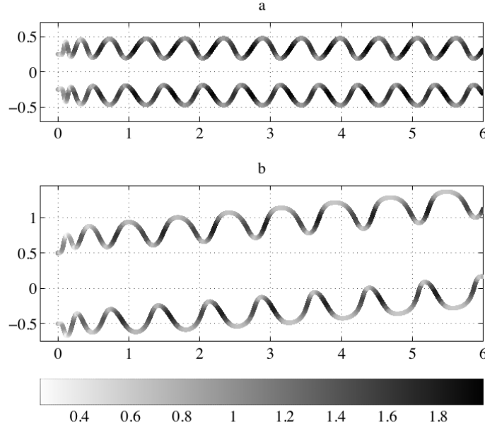
FIGURE 17. Droplet pair forming a stable ‘promenade mode’. Two identical droplets propagate together in a given direction while oscillating in the transverse direction. Axes are in units of the Faraday wavelength. Two walkers bouncing (a) in-phase, and (b) out of phase. The instantaneous speed V/C_p is color-coded according to the underbar. The mean speeds of the promenading pair in (a) and (b) are 0.88 and 0.63 of the single-walker free walking speed, respectively.
