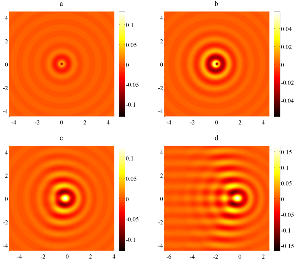
FIGURE 14. Wave fields accompanying bouncing and walking drops. (a) At \Gamma = 3.1 , the axisymmetric wave field of a bouncer arises. At (b) \Gamma = 3.3 , (c) \Gamma = 3.8 , and (d) \Gamma = 4.15 , walkers of progressively increasing speed arise, their wave fields being progressively more fore-aft asymmetric. Axes are in units of Faraday wavelengths, and the surface elevation (sidebar) is in units of drop radii. In all figures, the drop is at the origin and (except for a) moving to the right. The simulations were performed with drops of \Omega = 0.8 (i.e. R_0 = 0.38\text{mm} ), for \Gamma_W = 3.15 .
