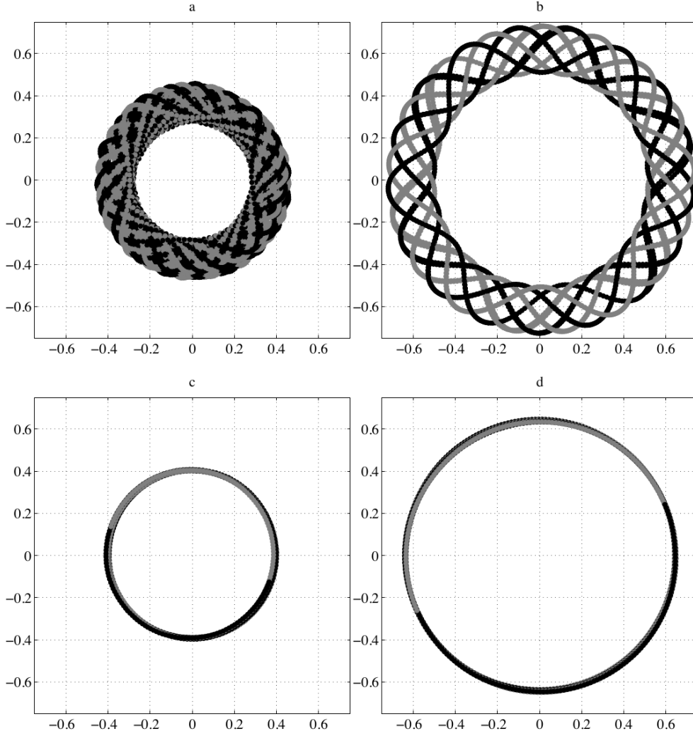
FIGURE 16. Orbital modes arising through walker-walker interactions, specifically from a pair of identical walkers launched with antiparallel velocity. Bouncing in phase with (a) c_4 = 0.32 , \Omega = 0.8 , \Gamma = 3.7 and (c) c_4 = 0.3 , \Omega = 0.7 , \Gamma = 4 . Bouncing out of phase with (b) c_4 = 0.32 , \Omega = 0.8 , \Gamma = 3.6 and (d) c_4 = 0.3 , \Omega = 0.7 , \Gamma = 4 . Axes are in units of the Faraday wavelength. Note the offset of orbital radii between the in- and out-of-phase walkers.
