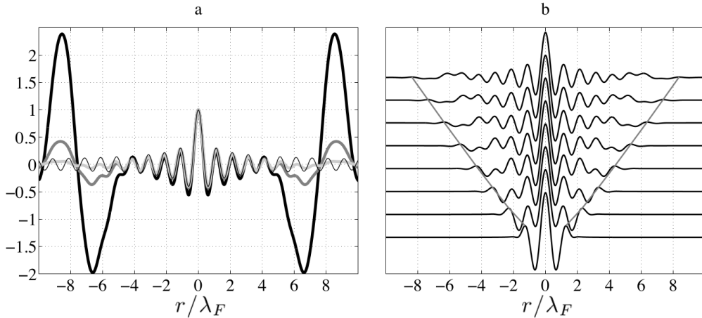
FIGURE 7. a) Cross sections of wave fields generated by single impact corresponding to panels b3 (black), c3 (grey), d3 (light grey) in figure 6, normalised to have the same height at the origin. The thin line corresponds to a Bessel function J_0(k_F r) . b) Cross sections of the single impact free surface for \Gamma = 4.15 at times t = T_F, 2T_F, \dots, 8T_F scaled so as to have the same height at the origin. The line indicates the leading edge of the disturbance. The horizontal axes show distance from the point of impact.
