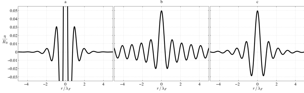
FIGURE 8. Different model predictions of the free surface cross section of a (2,1)^1 bouncer at the moment before impact with \Gamma = 3.1 . (a) The cosine wave model (3.9) of Eddi et al. (2011) with a spatial damping with decay length 1.6 \lambda_F reported by the authors. Note the singularity at r = 0 . (b) The Bessel model (3.10) of Moláček & Bush (2013b). (c) The result of our computation.
