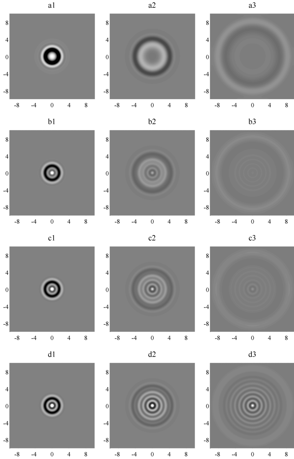
FIGURE 6. The computed wave fields generated by a single drop impact on a quiescent bath (a1-a3), and a bath vibrating at f = 80\text{Hz} with \Gamma = 3.15 (b1-b3), \Gamma = 3.6 (c1-c3) and \Gamma = 4.15 (d1-d3). The wave field was generated by a single impact of a drop of R_0 = 0.38\text{mm} and density ten times that of the bath. The axes are labelled in units of Faraday wavelengths. Images are taken at times t = 2T_F (a1-d1), t = 6T_F (a2-d2) and t = 11T_F (a3-d3) after impact, where T_F is the Faraday period.
