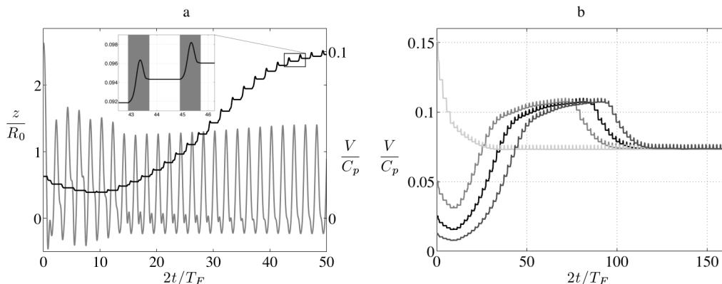
FIGURE 2. a) Evolution of the droplet’s horizontal velocity ( V/C_p , black) and elevation above the free surface ( z/R_0 , gray), in the bath’s frame of reference. Following its release onto the surface at a low speed, the droplet decelerates, then accelerates towards its steady walking speed. The inset shows the velocity variations over the Faraday period, reflecting the two stages of the drop motion, impact (grey) and free flight. b) Evolution of the walker dynamics from different initial conditions. After an initial transient, all walkers converge on an identical walking state with the same impact phase.
