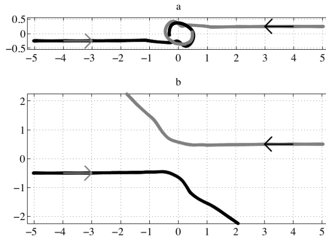
FIGURE 15. Collisions of in-phase droplet pairs. (a) With impact parameter of d_I = 0.5\lambda_F , the pair are captured in a periodic orbit with a diameter of approximately 0.5\lambda_F . (b) With an impact parameter d_I = \lambda_F , the droplets scatter. Vertical and horizontal length scales are in units of \lambda_F .
