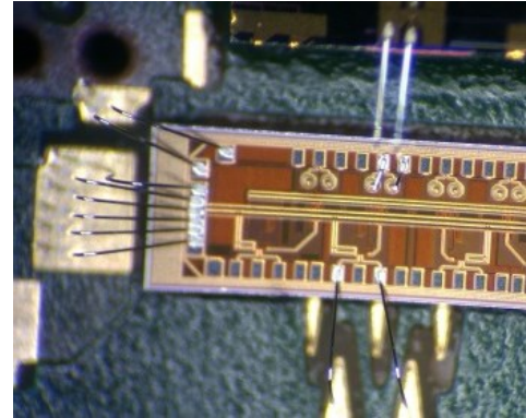
Fig. 12. Image of wire bonds between the CMOS transimpedance amplifier and the photodetector.
