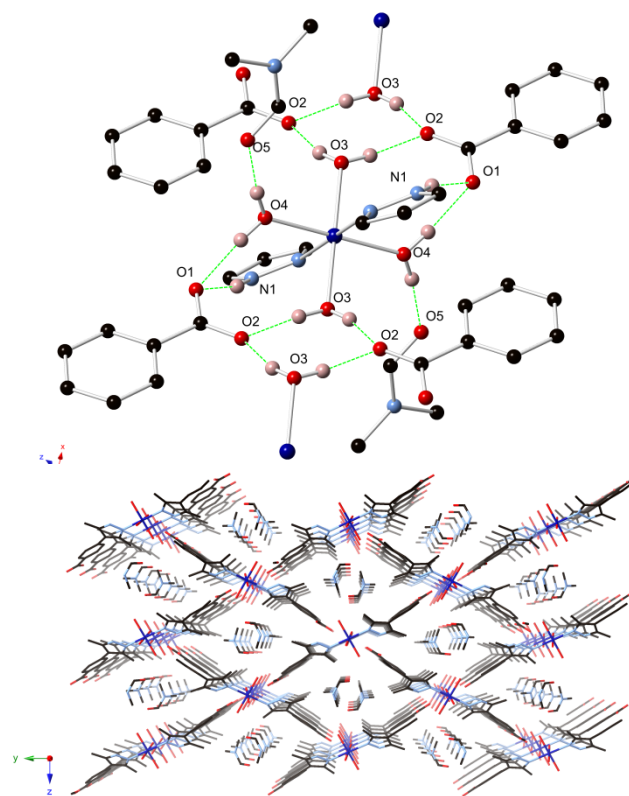
Figure 4 (a) The structure of the complexes in 1 with only selected hydrogen atoms shown; (b) A perspective view of the hydrogen bonding around the metal centres in 1 ; (c) A view down the a -axis of the rectangular channels containing DMF guests in 1 with hydrogen atoms omitted for clarity. Symmetry codes used to generate equivalent atoms: (i) -x, -y, 2-z .
