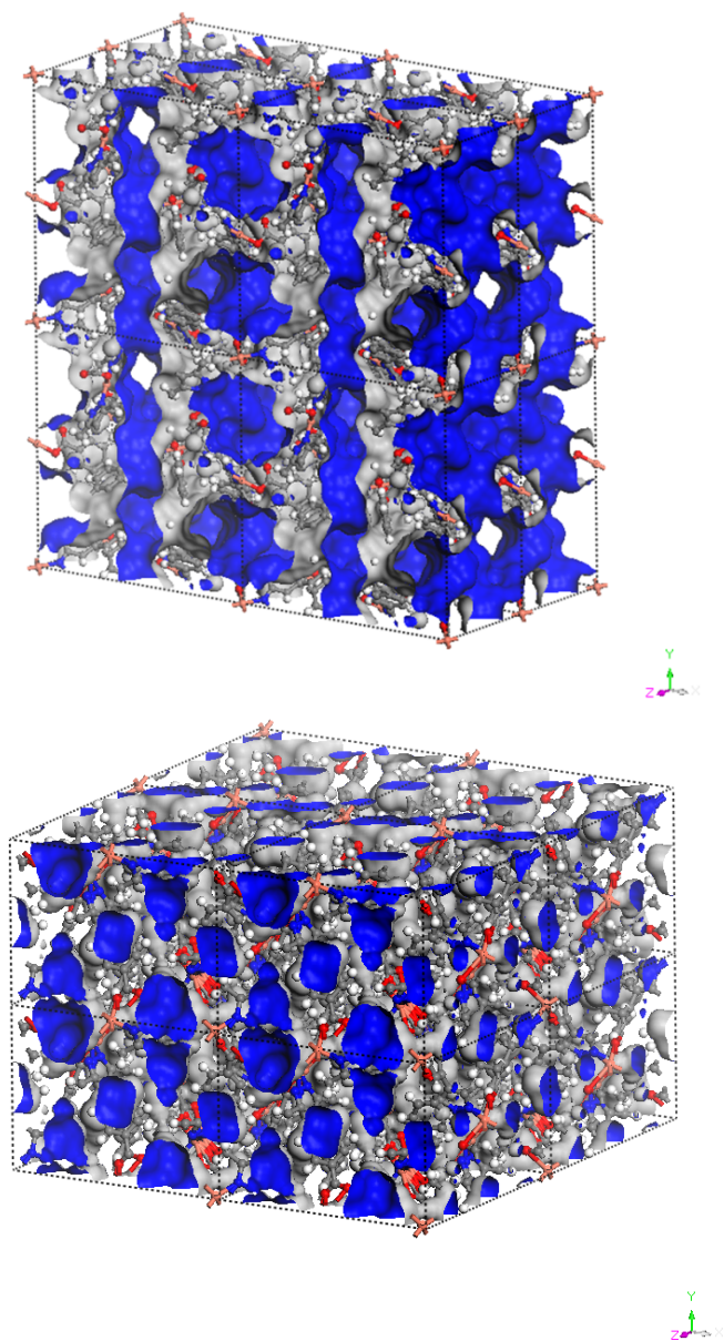
Figure 10 Perspective views of Connolly surfaces of 2 \times 2 \times 2 unit cells of 8 (top) and 8-dry (bottom) with solvate molecules removed to highlight the channels that exist in 8 and small solvent accessible areas in 8-dry .
