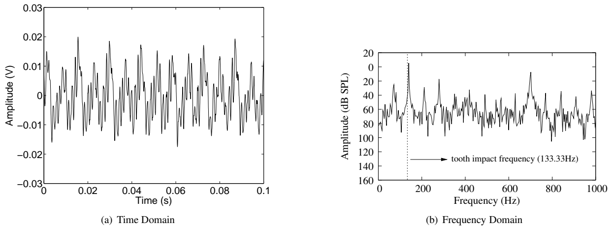
Figure 8: Time and frequency domain for signal estimate. The cutting parameters are: 4000rpm spindle speed, 1800mm/min feed rate, and 2mm depth of cut. In (b) the vertical dashed line indicates the theoretical tooth-impact frequency which corresponds to approximately to 133.33Hz.
