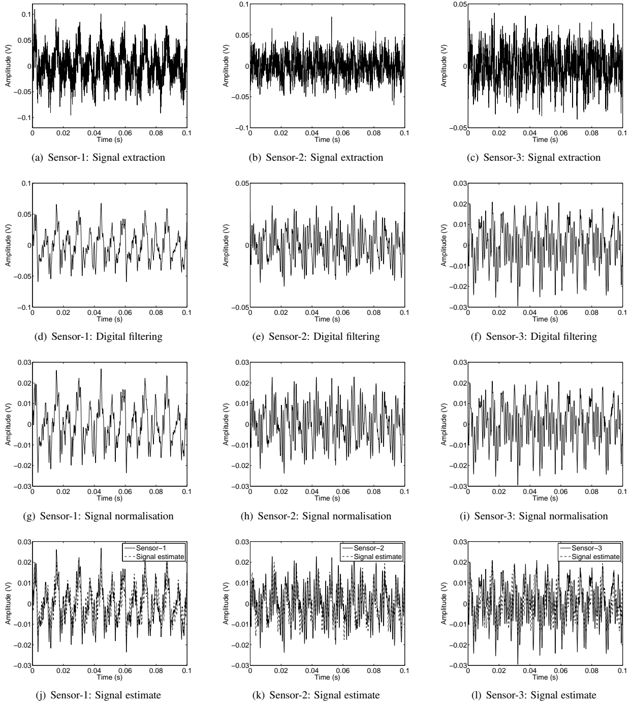
Figure 6: Demonstration of Framework 1 on a single set of machining parameters. The plots shows the signal waveform obtained along the framework steps. The cutting parameters are: 4000rpm spindle speed, 1800mm/min feed rate, and 2mm depth of cut.
