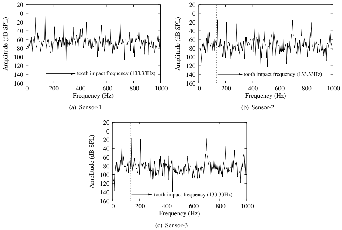
Figure 7: Frequency spectrum for Sensor-1, Sensor-2, and Sensor-3. The cutting parameters are: 4000rpm spindle speed, 1800mm/min feed rate, and 2mm depth of cut. The vertical dashed line indicates the theoretical tooth-impact frequency which corresponds to approximately to 133.33Hz.
