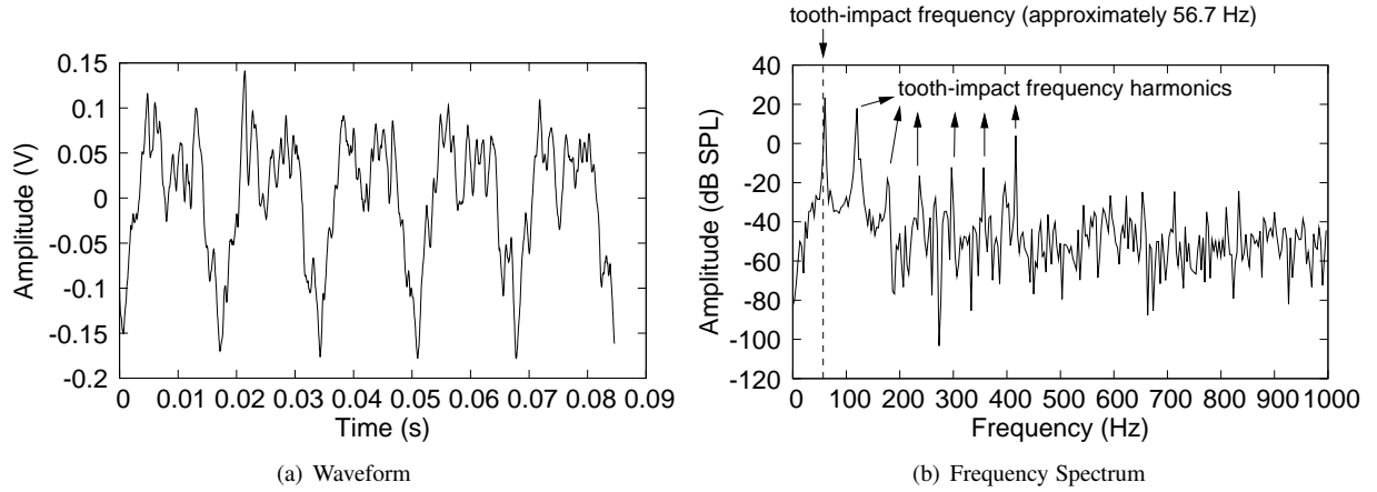
Figure 5: Acoustic transient signals captured during a milling operation. The signal as been captured by Sensor-1 and the cutting parameters are 1700rpm spindle speed, 510mm/min feed rate, and 4mm depth of cut. The signal has been filtered by a band-pass filter as detailed in Section 5.1. The vertical dotted line in (b) denotes the tooth-impact frequency.
