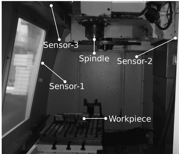
Figure 2: Position of the AE sensors, spindle and workpiece, inside the CNC milling machine.
