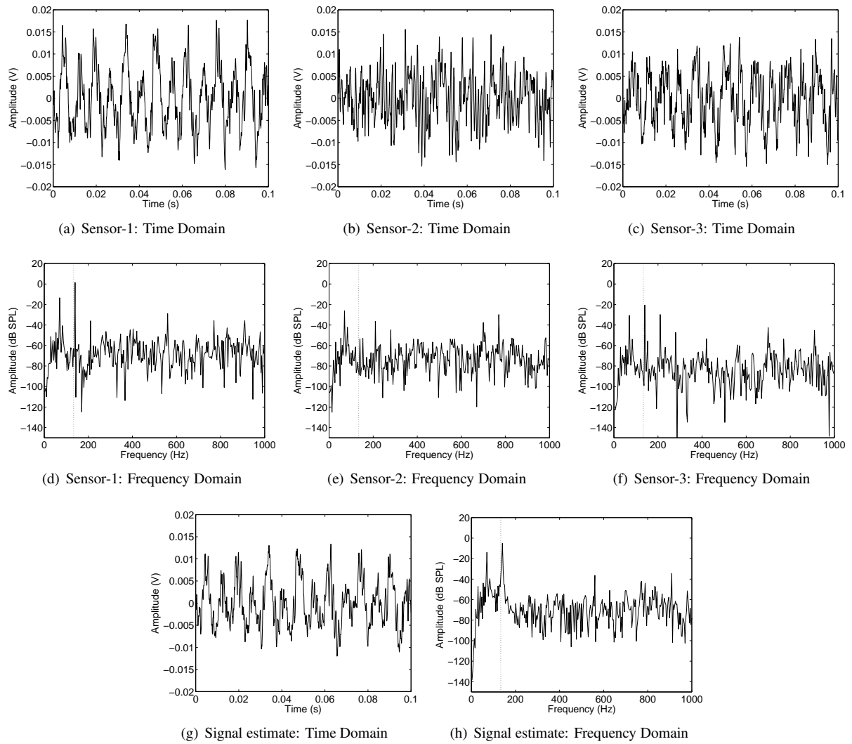
Figure 9: Time and frequency domain for Sensor-1, Sensor-2, Sensor-3 and signal estimate. The cutting parameters are: 4000rpm spindle speed, 1800mm/min feed rate, and 1mm depth of cut. In the frequency domain figures the vertical dashed line indicates the theoretical tooth-impact frequency which corresponds to approximately to 133.3Hz.
