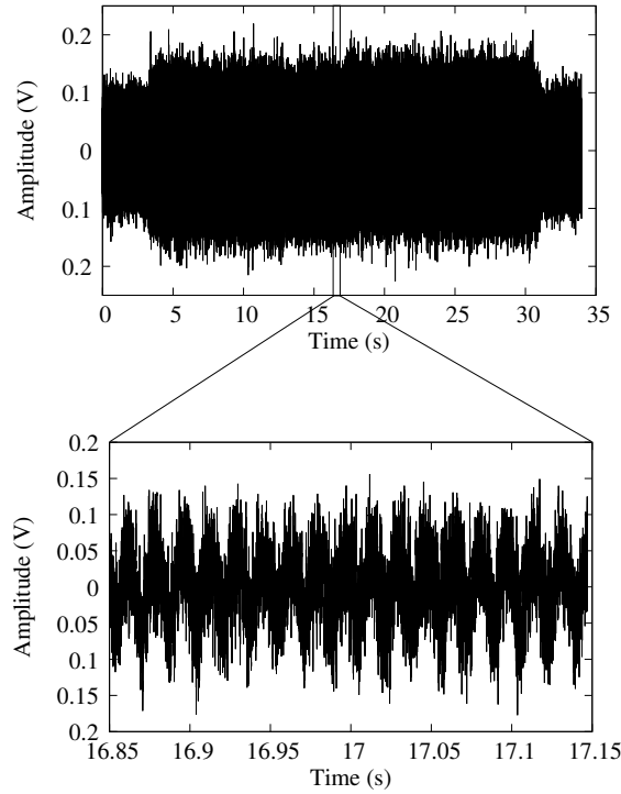
Figure 4: AE signal captured during a complete cutting operation is shown on top and the selected segment is shown on the bottom. Note that the signal segment selected corresponds to the time instant when the spindle is in the centre of the workpiece.
