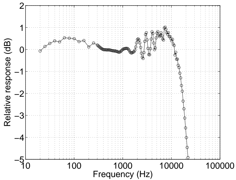
Figure 3: Frequency response for microphone Behringer ECM8000. The calibration data has been provided by Behringer upon request.
