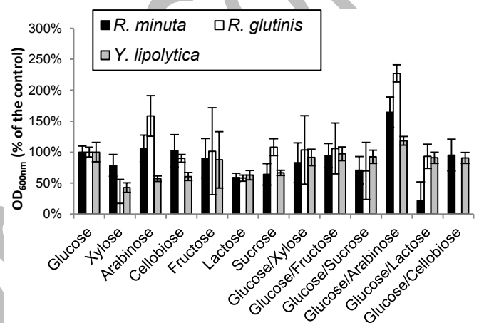
Figure 4 Cell mass productivity for R. minuta , R. glutinis and Y. lipolytica on a range of simple sugars, O.D. 600nm was taken at 120 h. The OD 600nm was standardised to a percentage of the growth on glucose. The yeast were cultured on 96 well plates at 28°C. The error bars show the standard deviation from 6 samples.
