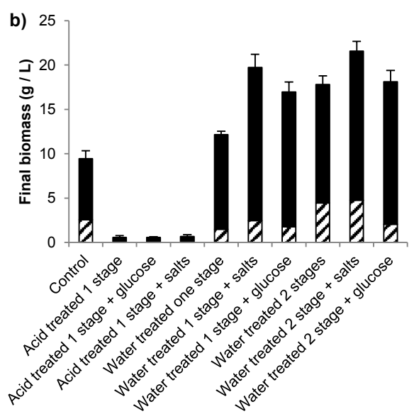
Figure 7 a) Sugar consumption for R. minuta cultured on municipal food waste depolymerised through a water treatment step (121 °C, 30 minutes). (b) Final cell mass and lipid (shaded) contents for R. minuta cultured on food waste depolymerised through an acid treatment (3% H 2 SO 4 , 121 °C, 30 minutes), a water treatment (121 °C, 30 minutes) and cultured in a 2 stage process where the yeast was cultured for 4 days on water treated food waste followed by a glucose-only stage for 2 days.
