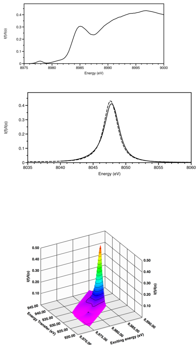
Fig 2 Cu K-edge XANES of CuO showing the HERFD spectrum (top), K\alpha_1 emission spectra of CuO (solid) and Cu (dashed) with the exciting energy above the absorption edge a (middle) and K\alpha_1 RIXS. Data recorded on I20 of the Diamond Light Source.
