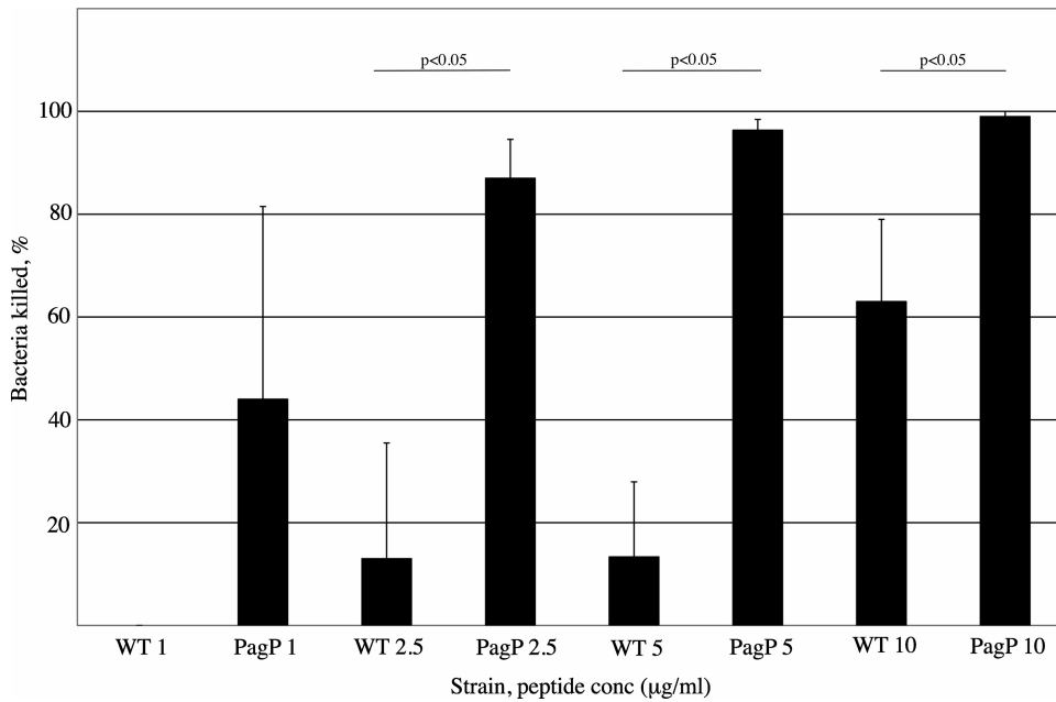
FIG 5 B. paraptertussis pagP is more susceptible to killing by the synthetic antimicrobial peptide C18G than the WT. A significantly different level of killing of the WT compared to the pagP mutant was observed. This was observed in three independent experiments; data from a representative experiment are shown here.
