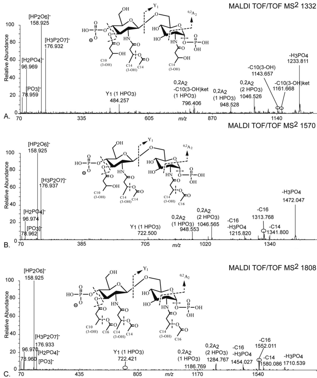
FIG 3 Negative-ion-mode MALDI-TOF/TOF mass spectra for precursor ions at m/z 1,332 (A), m/z 1,570 (B), and m/z 1,808 (C) isolated from WT B. paraperussis lipid A. Proposed lipid A structures for each precursor ion are shown in each spectrum, with dashed lines representing possible cleavage sites. Diagnostic cross-ring and glycosidic product ions provided unambiguous structure assignment and were named according to the nomenclature outlined by Domon and Costello (29), with the slight modification of designating the number of phosphate groups present and the loss of neutral acyl chains if applicable. All precursor ions were diphosphorylated with a heterogeneous mixture of bisphosphate and pyrophosphate. Only the bisphosphate configuration is displayed. C 16 , palmitic acid; C 10 (3-OH), 3-hydroxy capric acid; C 10 (3-OH)ket, neutral loss as a ketene; HPO 3 , phosphate; H 3 PO 4 , phosphoric acid; [H 3 P 2 O 7 ] - and [HP 2 O 6 ] - , pyrophosphate product ions; [H 2 PO 4 ] - and [PO 3 ] - , phosphate product ions.
