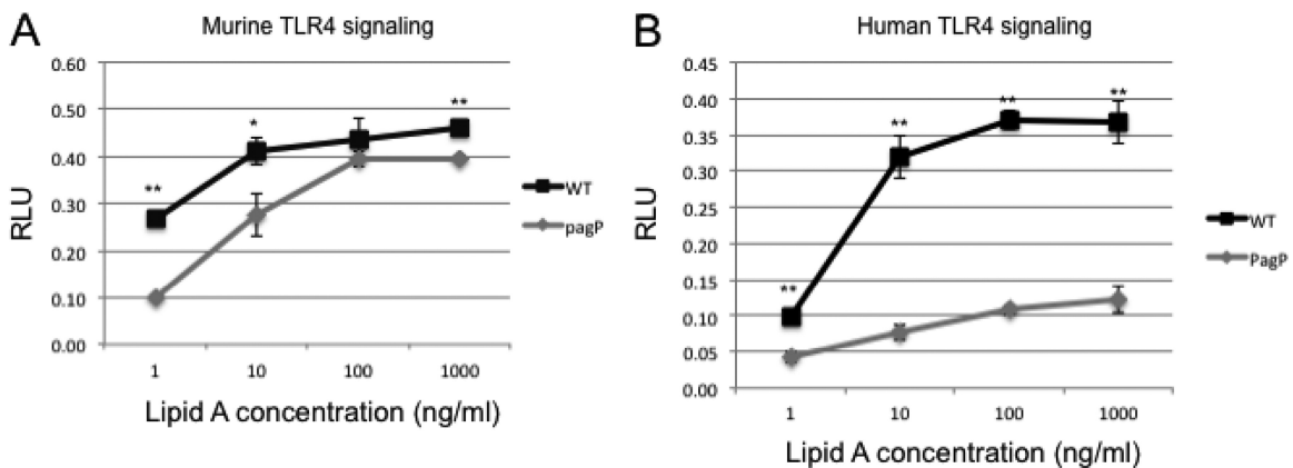
FIG 6 Stimulation of murine or human TLR4-mediated signaling by WT and B. paraptertussis lipid A. Both lipid A's were more potent stimulators of murine than of human TLR4-mediated signaling; however, B. paraptertussis pagP lipid A was significantly less potent than that of the WT, particularly for the activation of human TLR4. *, P < 0.05; **, P < 0.001.
