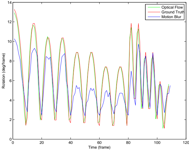
Shutter Angle and Rotation Estimates from a Synthetic Dataset (Synthetic Box Sequence)
