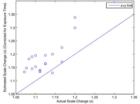
Figure 7: Results for Estimating Change in Focal Length from Blur with a Synthetic Data Set
