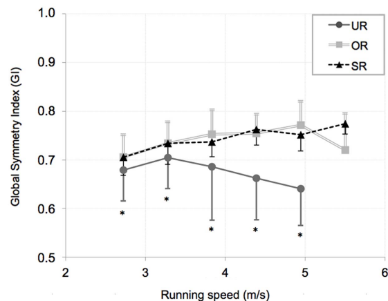
Figure 4. Mean values for the dynamic Global Symmetry Index (GI) plotted against running speed. Mean values for the dynamic Global Symmetry Index (GI) are evaluated starting from the single values of \overline{SI^x} , \overline{SI^y} and \overline{SI^z} and averaged within each group of subjects, \pm SD, in untrained runners (UR), occasional runners (OR) and skilled runners (SR). Two-way ANOVA (group \times running speed) show that the group of UR had a mean GI always lower compared to the OR and SR, ( * = p < 0.01 ), independently from the running speed. doi:10.1371/journal.pone.0074134.g004
