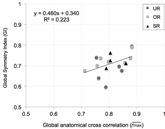
Figure 3. Regression of the mean dynamic Global Symmetry Index (GI) versus the global anatomical cross correlation value ( r_{max} ). Each point represents the mean Global Symmetry Index averaged among the different running speeds for each subject; Untrained Runners (UR), Occasional Runners (OR) and Skilled Runners (SR) ( r = 0.473 ; p = 0.055 ). doi:10.1371/journal.pone.0074134.g003
