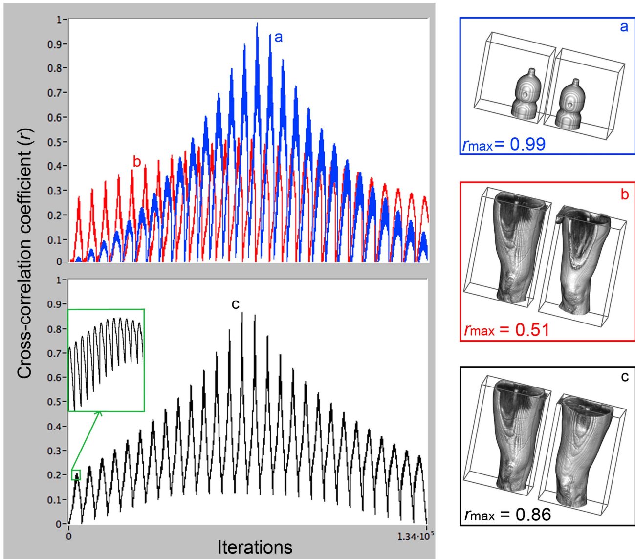
Figure 2. Examples of obtained cross-correlation values plotted versus iterations. Cross correlation values ( r ) of all iterations (134,400 overlap positions = 28 (i) × 60 (j) × 80 (k), between right volume and left reflected volume); a) comparison between two bottles, filled with the same volume of water ( r_{\max} = 0.99 ); b) comparison between the right upper leg of a subject and the left upper leg of a different subject ( r_{\max} = 0.51 ); c) comparison between right and left upper legs of the same subject. Inset: enlargement of cross correlation pattern showing the inner processing loop (i coordinates).
