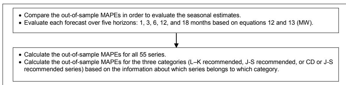
Fig. C.4. Accuracy Assessment
