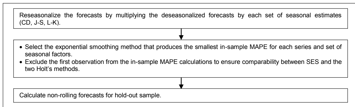
Fig. C.3. Prediction
