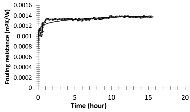
Fig. 9 Fouling resistance data of \text{CaCO}_3 and model fit (stainless steel probe)
