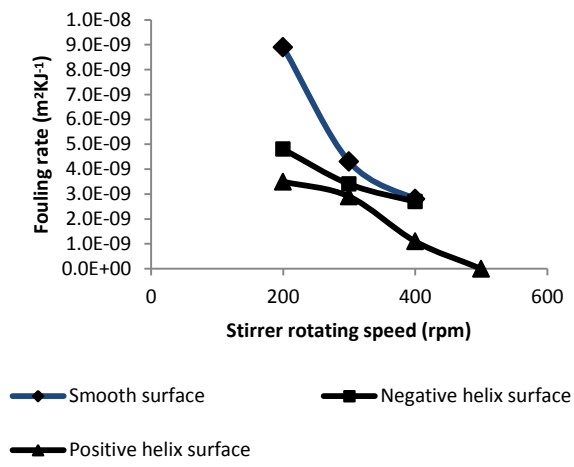
Fig. 13 Fouling rates of CaCO 3 on smooth, negative and positive helical surfaces
