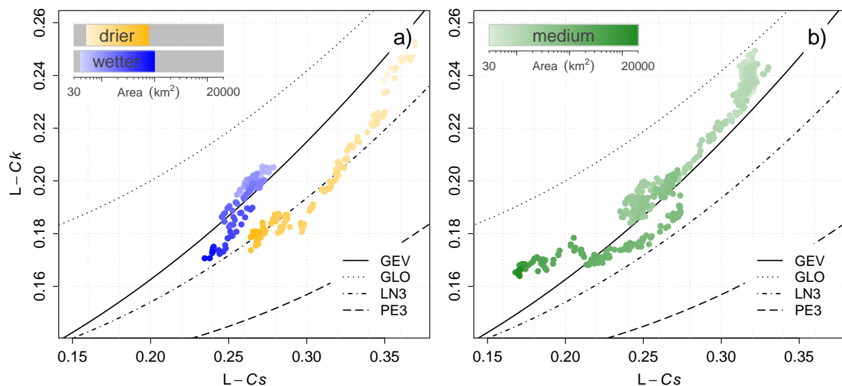
Figure 6. L-moment ratio diagrams for the subsets defined by MAP: (a) drier, wetter, and (b) medium described in Fig. 3. Each point represents the record length WMA over 70 catchments of L-Ck against corresponding values of L-Cs and the colour intensity is proportional to catchment area.
