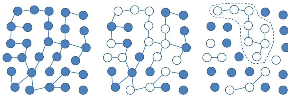
Figure 2. Percolation. In a random network ( left ), white nodes are willing to buy ( p_r > p ) and filled nodes are unwilling to buy ( p_r < p ) ( middle ). Widespread diffusion happens if an initial adopter is part of a giant connected component (surrounded by dotted lines) in the resulting “operational network” ( right ).
