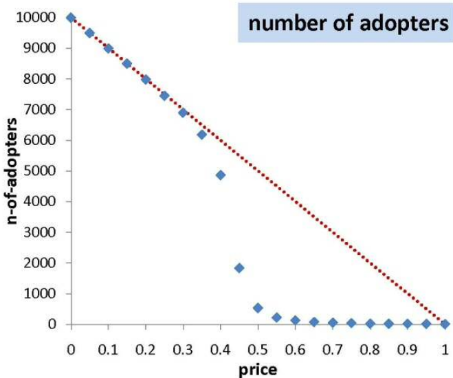
Figure 3. Percolation shows a critical transition.
