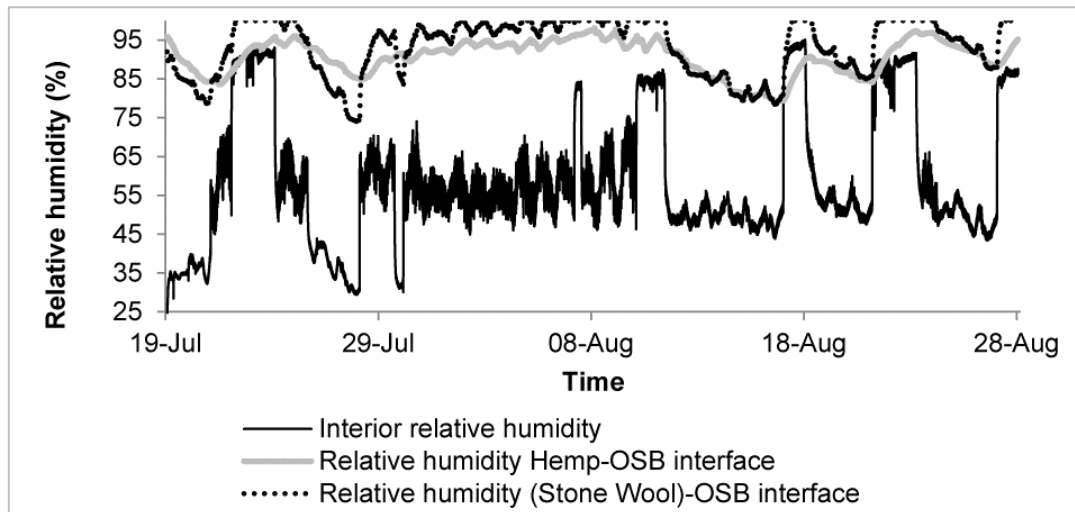
Fig. 15. The relative humidity conditions at insulation-OSB interfaces.
