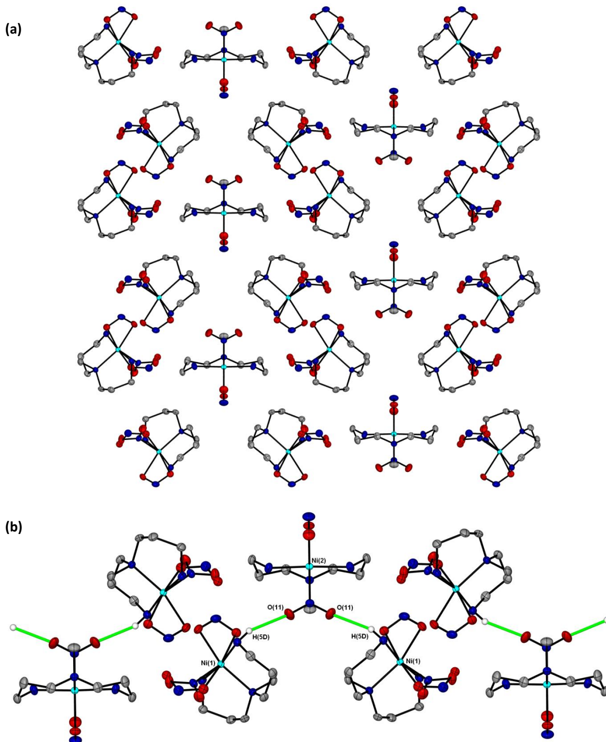
Figure 2. (a) Crystal packing arrangement for the structure of 1 at 298 K, (b) hydrogen bonding interactions to the nitro- (\eta^1\text{-NO}_2) ligand in molecule (B).
