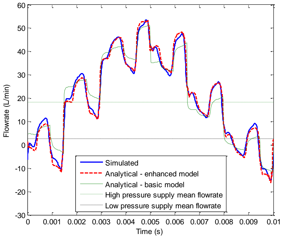
Figure 7 Simulated and analytical inlet flowrate of the inertance tube. Mean supply flowrates for the enhanced analytical model are also shown.
