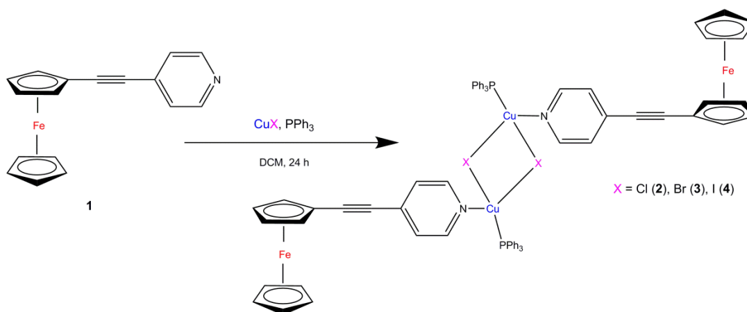
Scheme 1. Synthesis of neutral di-ferrocenyl-ethynylpyridinyl triphenylphosphine copper complexes
