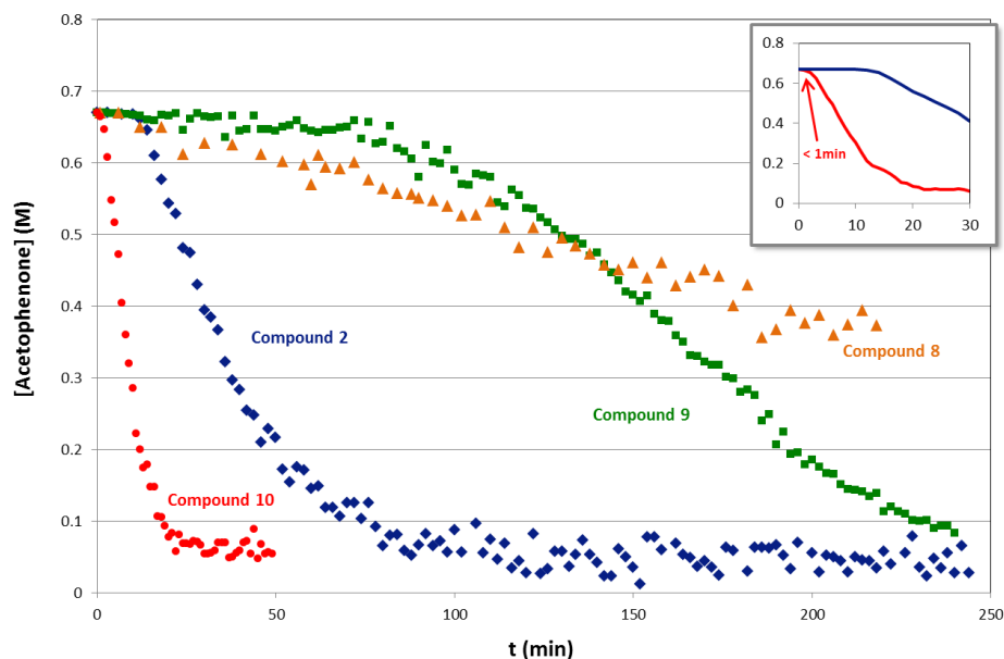
Figure 10. Profiles of acetophenone consumption monitored by ^1\text{H} NMR in the transfer-hydrogenation-reaction catalyzed by 2 ( \blacklozenge ), 8 ( \blacktriangle ), 9 ( \blacksquare ) and 10 ( \bullet ) in i\text{PrOH} (60 ^\circ\text{C} , 1 mol % [\text{Ir}] , 10 equiv. KOH, TMB as internal standard).
