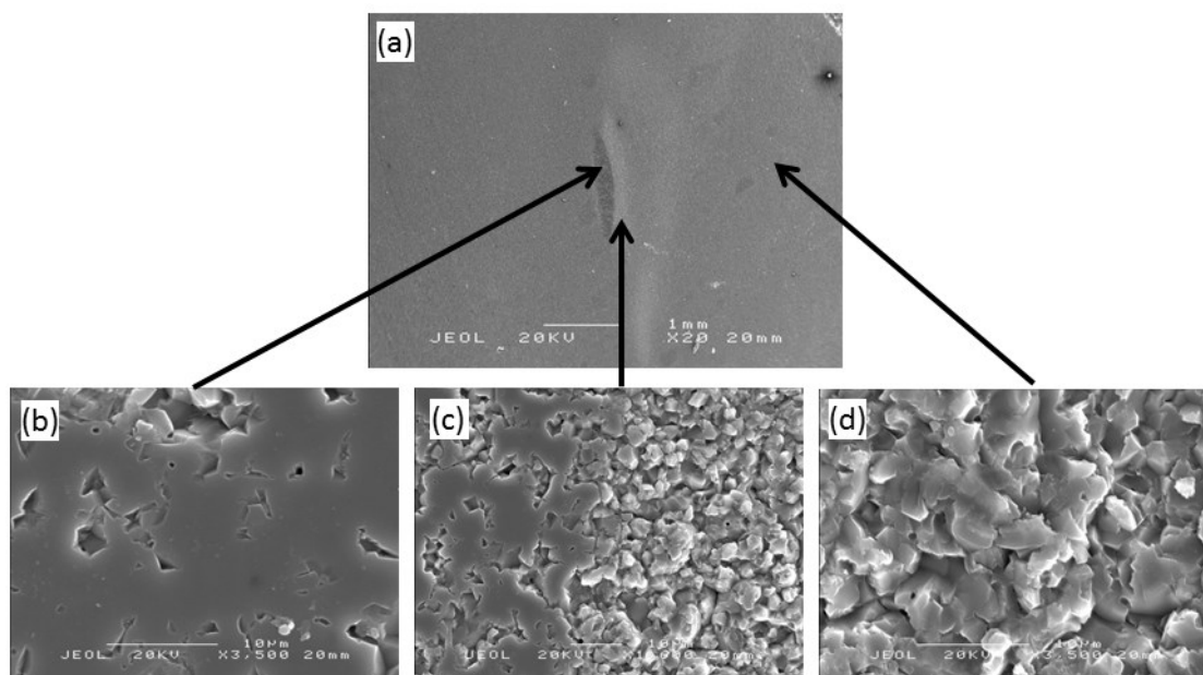
Figure 6. Scanning electron micrographs of hydroxyapatite after 15 min contact with tip A operating at full power (a) magnification \times 20 ; (b) contact area, magnification \times 3500 ; (c) boundary of contact area, magnification \times 500 ; (d) untreated area, magnification \times 3500 .
