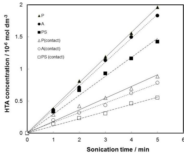
Figure 3. Production of OH radicals monitored by terephthalate dosimetry. The descalers were operated at full power; ‘contact’ signifies that the tips were placed against a glass slide.
