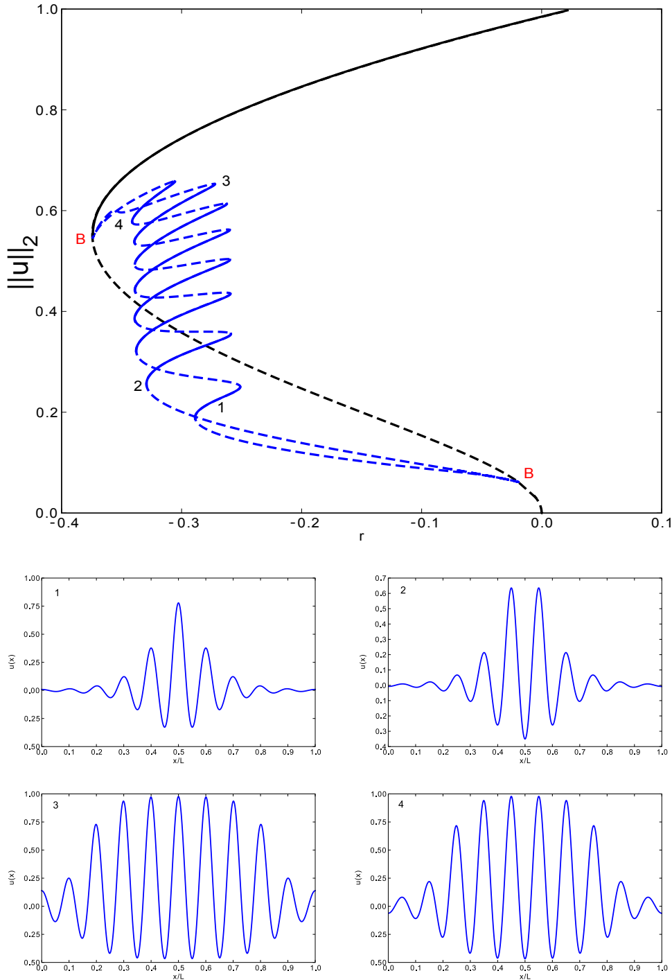
Figure 1: Homoclinic snaking for the SHE. Upper panel: bifurcation diagram showing branches of periodic patterns (black) and localised states (blue) in the (r, \|u\|_2) -plane for the N_{23} SHE, for b = 1.8 . Solid (dashed) lines indicate stable (unstable) solutions. Points marked ‘B’ are the bifurcations at which the localised states emerge from the periodic states and are a consequence of the finite computational domain. Lower panels: illustrative solution profiles u(x, t) at the four numbered locations on the bifurcation diagram. The domain length used is 0 \leq x \leq 20\pi , with periodic boundary conditions. This figure, and several others, was computed using the continuation software AUTO [14].
