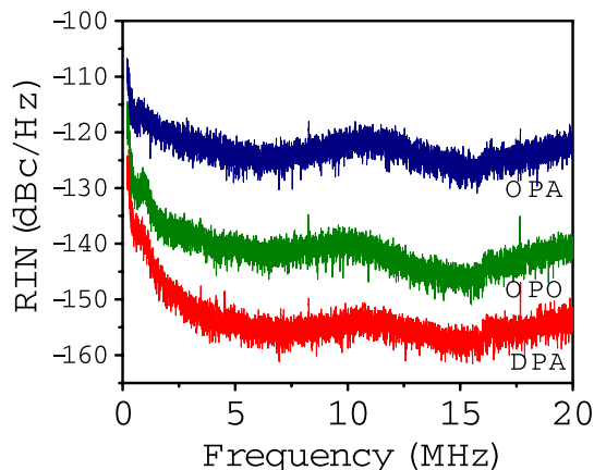
Fig. 6. Megahertz RIN measurement on fiber sources for coherent Raman microscopy taken with a resolution bandwidth of 6.5\text{ kHz} . The OPA measurement references the work done in [9].
