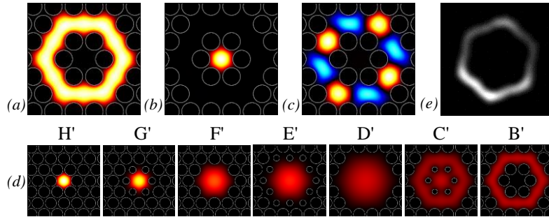
Fig. 7. (a)–(c) Calculated fields at B, for (a) the fundamental mode, (b) the 10th mode and (c) the 9th mode. (d) Simulated fields at locations H'–B' along a reverse mode converter, for an LP 01 input at H' (Media 2). An LP 02 input at H' would give the reverse of Fig. 6(a). (e) Experimental near-field pattern at the end of a reverse transition H'–B', for input light of wavelength 800 nm in the LP 01 mode at H'.
