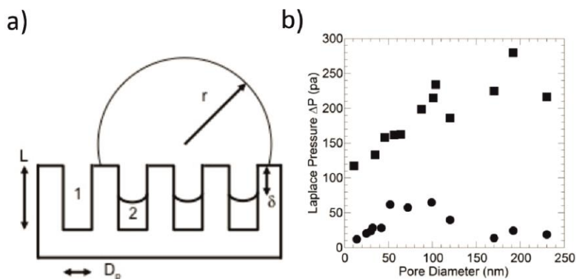
Fig. 3. (a) Schematic of water droplet penetration inside cylindrical channels of length L and diameter D_p for a silanized, hydrophobic, PAA. The liquid penetrates inside the pores by a depth \delta \leq L , as a function of water drop diameter, r and pressure of air trapped inside the pore. (b) Laplace pressure of water droplets on silanized (■) and bare (●) PAAs as a function of pore diameter.
