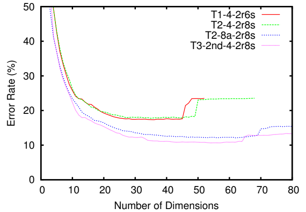
Figure 5. Variation of error rate with the number of PCA bases.
