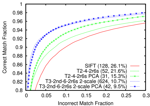
Figure 6. ROC curves for selected descriptors: Notre Dame. Figures in brackets show dimensionality and error rates.
