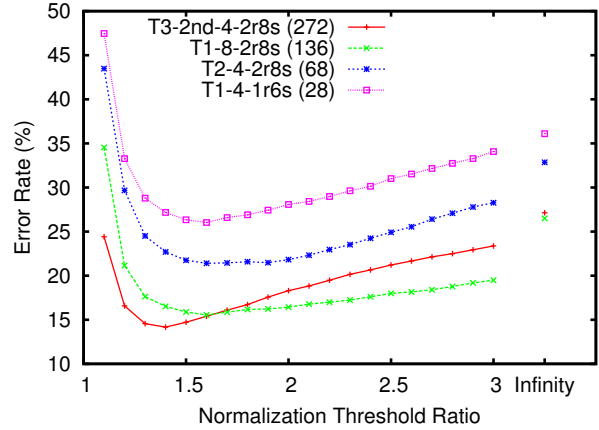
Figure 4. Variation of error rate with normalization threshold (Notre Dame). The threshold was set to r/\sqrt{D} where r is the ratio and D is the descriptor dimensionality (given in brackets).
