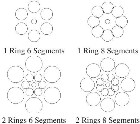
Figure 2. Typical DAISY descriptor Gaussian summation regions learned by our algorithm for steerable filter T-blocks. Circles indicate 1 standard deviation. Best results were obtained by offsetting concentric rings by 180/n degrees, where n is the number of segments.
