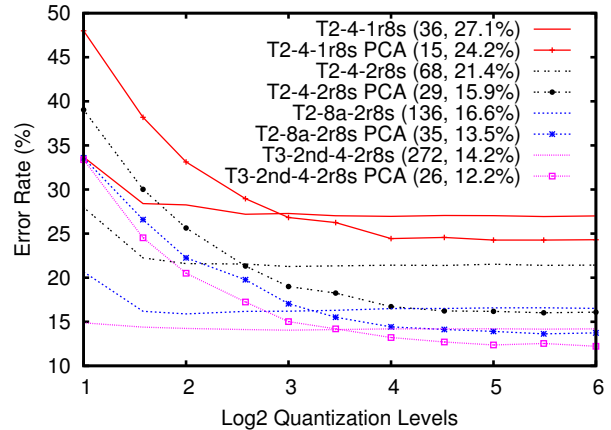
Figure 7. Quantization of descriptor dynamic range: Notre Dame. Error rate reduces rapidly as the number of levels used to represent the descriptor elements is increased from 2^1 to 2^6 . Figures in brackets show dimensionality and error rates.
