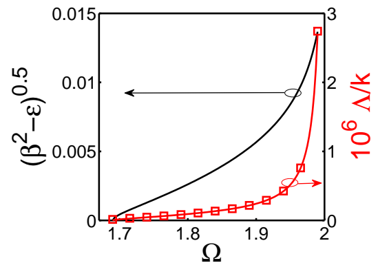
FIG. 6: (Color online) Dispersion of TE plasmon in the silicon-graphene-silicon geometry: Plasmon localization factor q = \sqrt{\beta^2 - \epsilon} , propagation loss \Delta/k and imaginary part of the propagation constant (squares).
