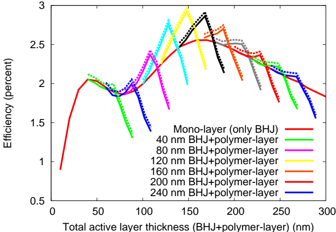
Figure 9: A plot of device efficiency against total active layer thickness (BHJ+polymer layer). The red line stretching from 10 nm to 300 nm shows a device with no polymer layer consisting of a BHJ only. The other lines represent devices formed from BHJs of different set thicknesses (40nm, 80nm, 120nm, 160nm, 200nm and 240nm) with varying thickness polymer-layers added to the structures. It can be seen that the addition of pure polymer layer with a thickness matching the exciton diffusion length can significantly increase device efficiency. The dotted lines show the impact of increasing the shunt resistance from 3 \times 10^4 \Omega to 1 \times 10^6 \Omega .
