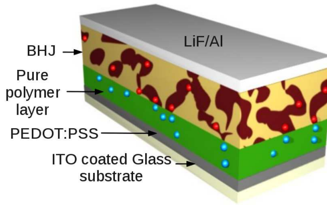
Figure 1: A diagram of the more efficient bi-layer structure. A polymer layer is used to replace a 30 nm section of the BHJ. This reduces the amount of fullerene used and increases solar cell efficiency. The blue spheres represent holes and the red spheres represent electrons.
