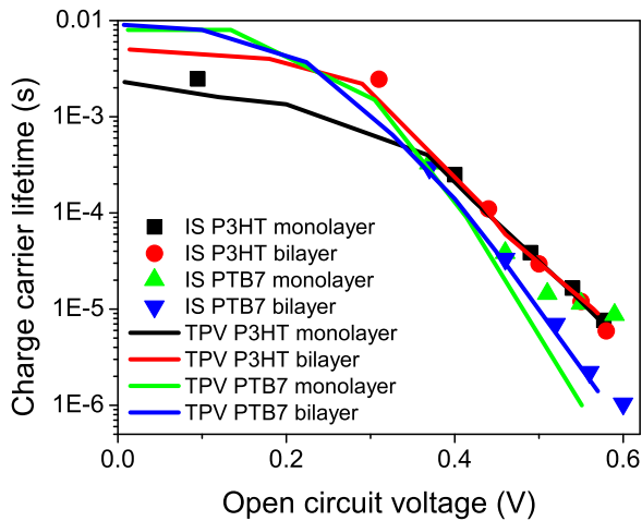
Figure 3: Carrier lifetimes measured by TPV and IS for P3HT:PCBM and PTB7:PCBM systems.
