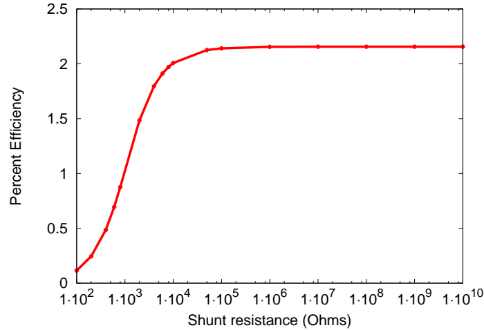
Figure 7: Device efficiency plotted against shunt resistance. The mono-layer devices have a low shunt resistance, this was boosted with the introduction of the bi-layer.
