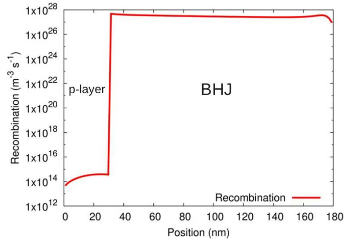
Figure 10: Recombination as a function of position within the device at V_{oc} . There is very little recombination within the p-layer due to the heterojunction at the polymer/BHJ interface.
