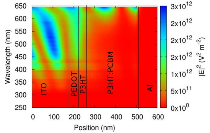
Figure 6: The photon distribution within the devices as a function position and wavelength.
