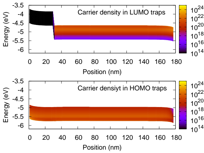
Figure 5: Energy and position space plot of carrier density within the simulated device. The polymer layer can clearly be seen on the left hand side of the device. It can be seen that the pure polymer layer has a very low electron density.
