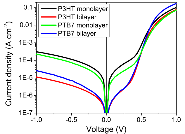
Figure 4: Dark JV curves for the mono-layer and bi-layer structures made from P3HT:PCBM and PTB7:PCBM. The polymer layer increases the shunt resistance.
