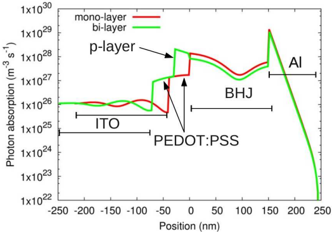
Figure 8: The photon absorption within the device as a function of position summed over the spectrum. It can be seen that a significant amount of light is absorbed in the pure polymer layer, therefore, for the bi-layer devices to have an increased efficiency the excitons generated within this layer must be split and reach the contacts as current.
