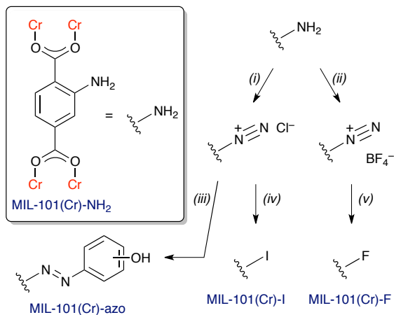
Scheme 1. Tandem post-synthetic modification of MIL-101(Cr)-NH 2 . (i) NaNO 2 , HCl (aq); (ii) NaNO 2 , HBF 4 (aq); (iii) C 6 H 5 OH (aq), Na 2 CO 3 ; (iv) KI (aq); (v) 100 °C.
